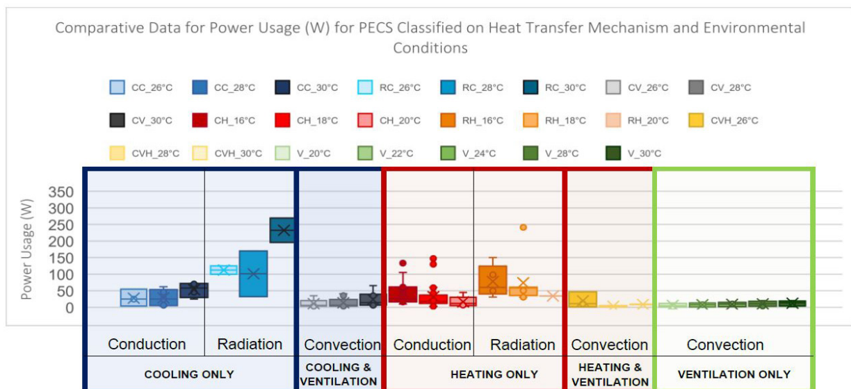
Figure 4 Power Usage Data Comparative Summary for all PECS types at given ambient temperatures (CC- Conductive Cooling; RC- Radiative Cooling; CV- Convective Cooling; CH- Conductive Heating; RH- Radiative Heating; CVH- Convective Heating; V- Ventilation)
