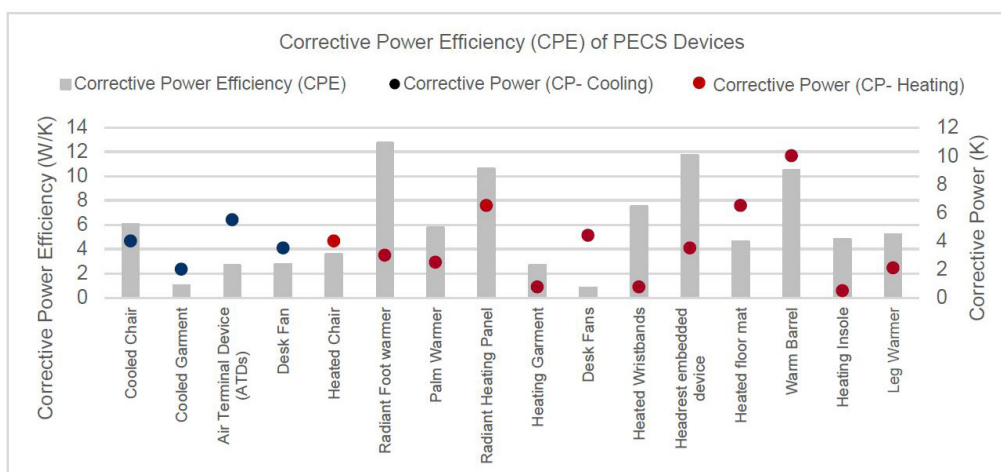
Figure 5 Corrective Power Efficiency data for PECS device applicability
