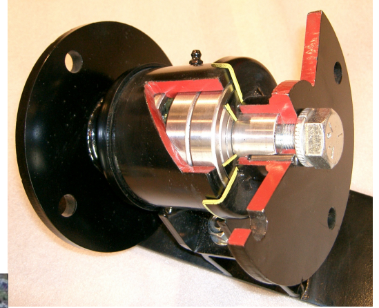
Coultter Kit cut away
