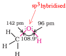
Methanol
