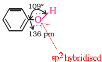
Phenol
