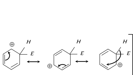
Resonance forms of carbonium ion (Arenium ion)
