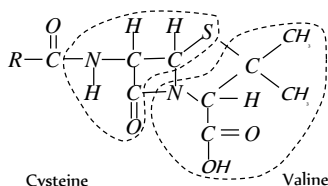
General structure of penicillin
