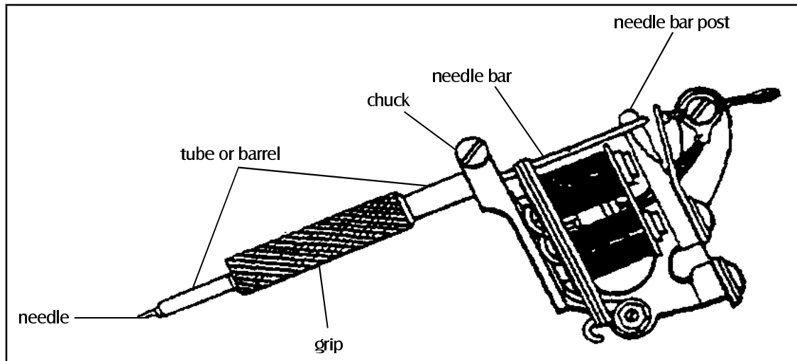
Figure 1 The Tattoo Machine*
