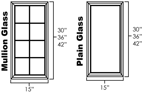
MD (Mullion)
