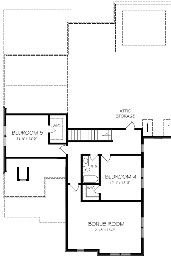
SECOND FLOOR PLAN 2 BEDROOMS
