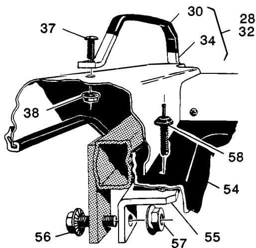
FENDER AND BAGWELL DETAILS
