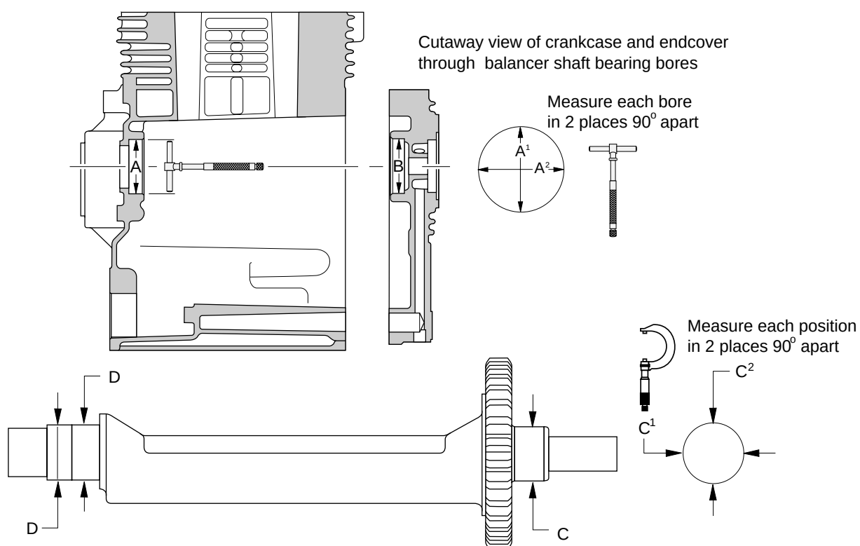
Fig. C-6 Balancer Shaft Journals, Gear and Bearing Bores
