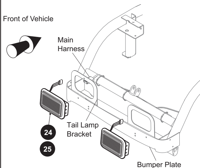
Tail Lamp Installation for vehicle without Flip Seat
