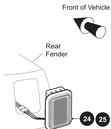
Tail Lamp Installation for vehicle with Flip Seat
