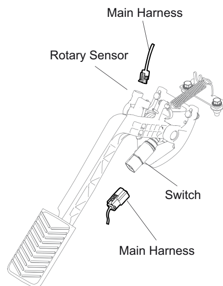
Accelerator Wiring Connection
