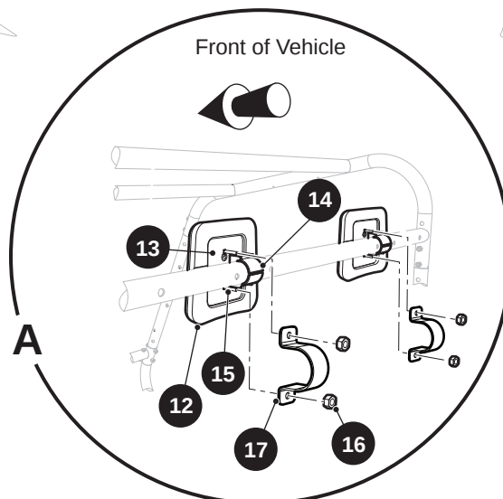
VIEW A, FROM REAR OF THE VEHICLE
