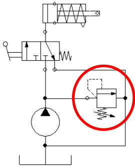
System Relief Valve 1, 2
