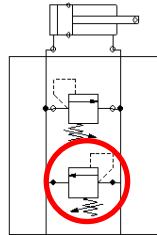
Cross Over Relief Manifolds 1, 2, 4, 5
