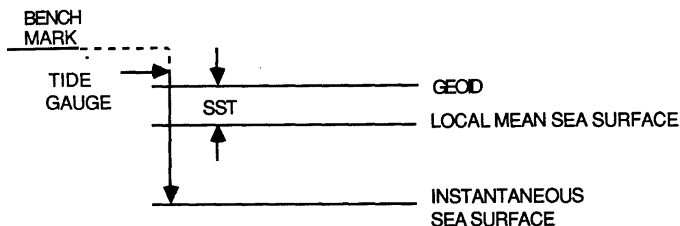
Figure 3.7. Measurements at a tide gauge site.
