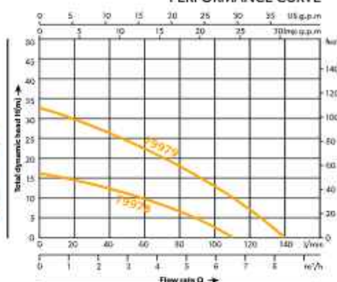
PERFORMANCE CURVE
