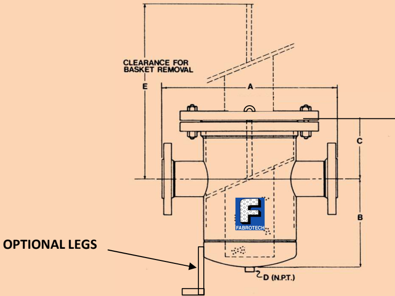
MODEL H-150/H-300: BUTTWELD
