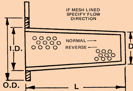
MODEL "B" CARBON STEEL MODEL "BS" STAINLESS STEEL BASKET TYPE
