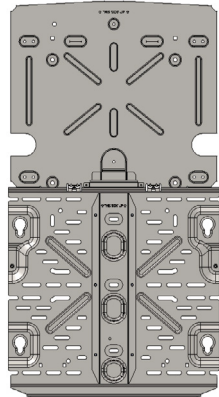
Wall-mount brackets
