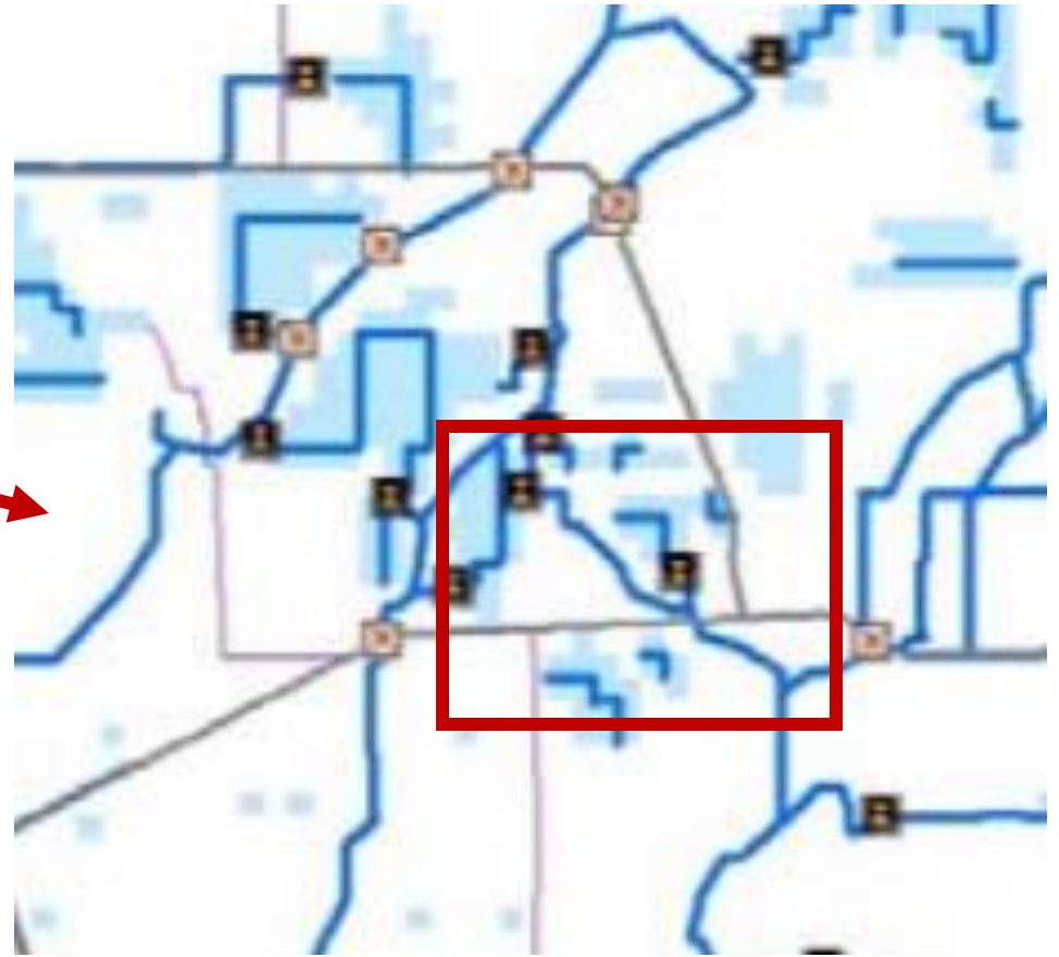
Figure 24: Networks & Structures
