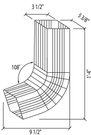
ROLL FORMED DOWNSPOUT (72° KICKOUT)
