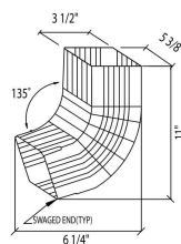
ROLL FORMED DOWNSPOUT (45° OFFSET)
