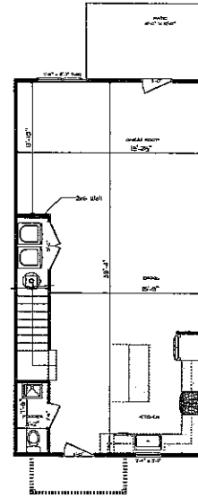
PLAN C REVERSED 1,600 SF 3 BR/ 2.5 BA
