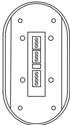
G8NB Detector Base
