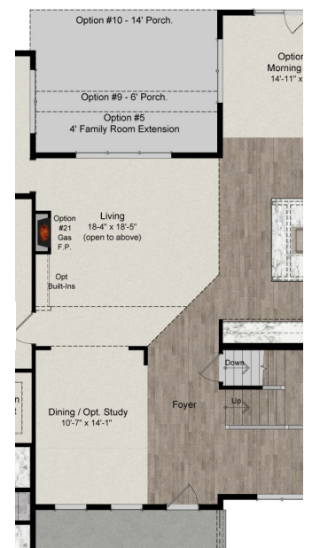
Family Room & Porch Extension
