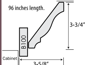
A141 ANGLED CROWN MOULDING
