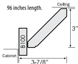
A140 ANGLED CROWN MOULDING
