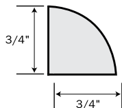
A104 BASE SHOE (Use for Both Base and Scribe)
