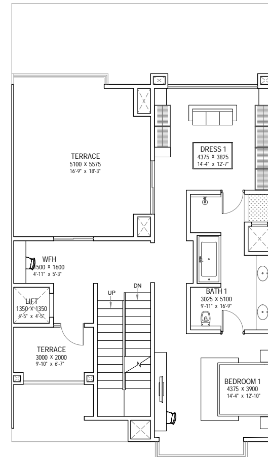
THIRD FLOOR
