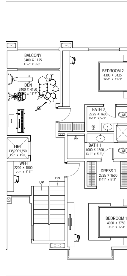
THIRD FLOOR
