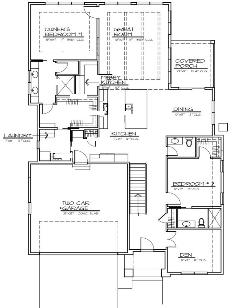
FIRST LEVEL FLOOR PLAN
