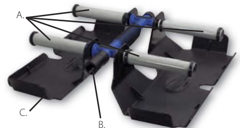
ProAir 4 For Ponds And Lakes Diffuser Size: 19"L x 19"W x 5"H
