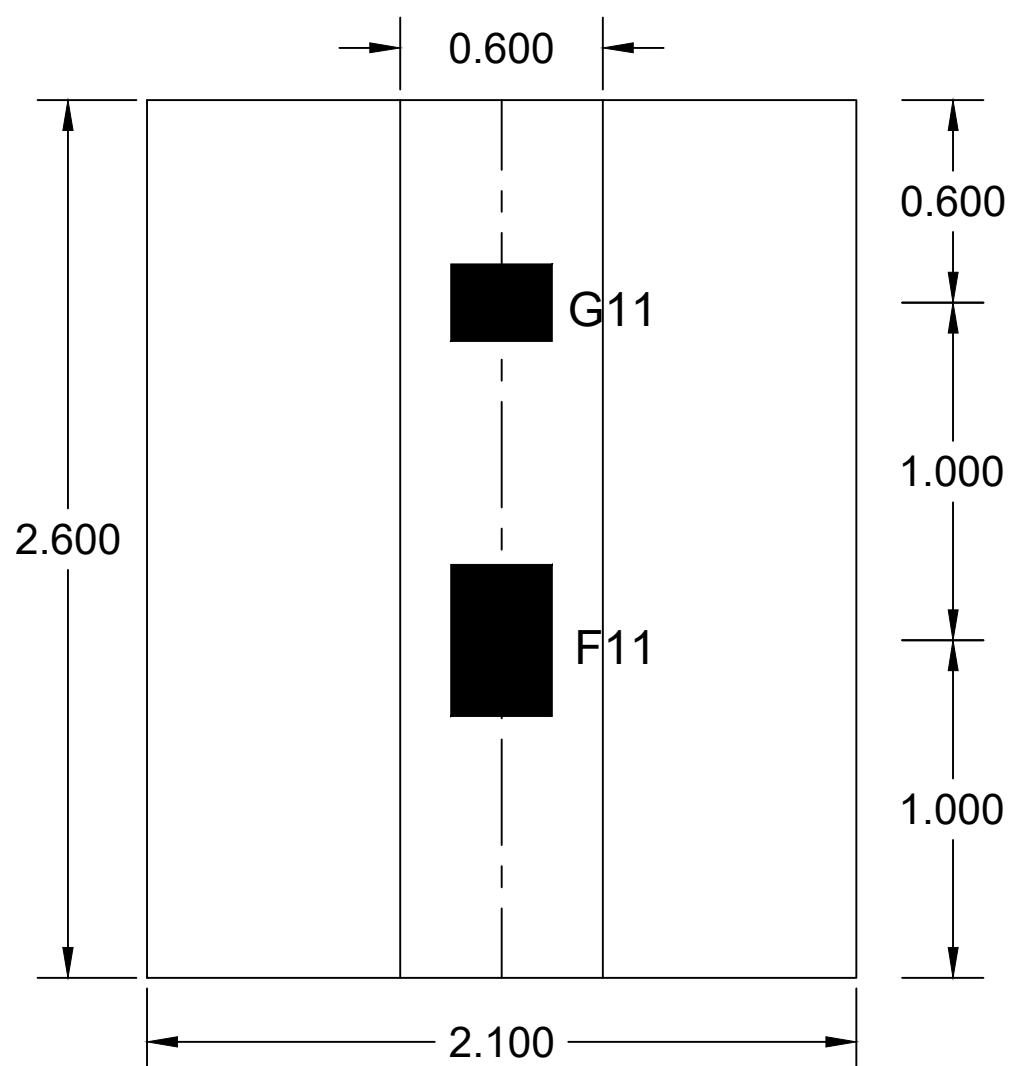
COMBINED FOOTING FOR COLUMNS F11-G11
