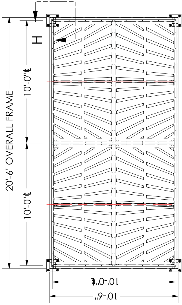
TOP VIEW SCALE 1 / 55
