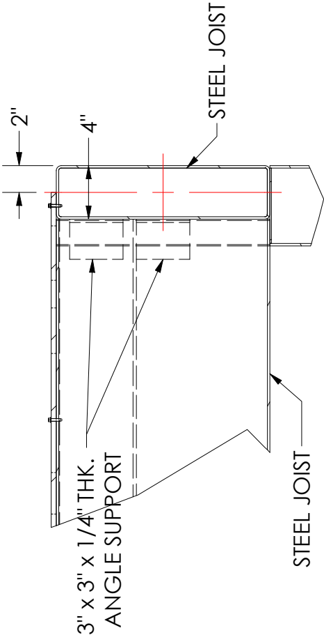
SECTION VIEW K SCALE 1/13
