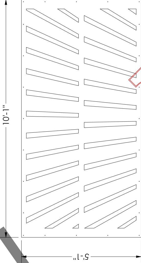
PANEL C SCALE 1 / 25
