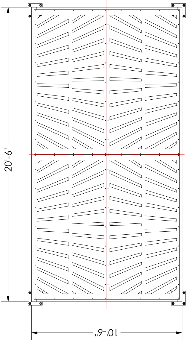
TOP VIEW SCALE 1/4" = 1'
