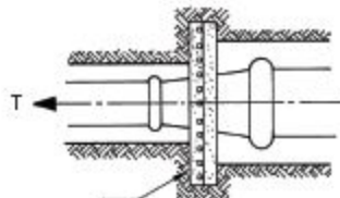
Concrete thrust wall set into undisturbed material in the trench wall
