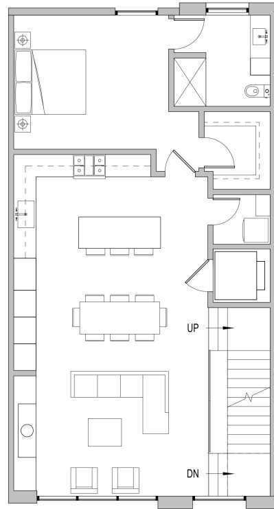
LEVEL 2
