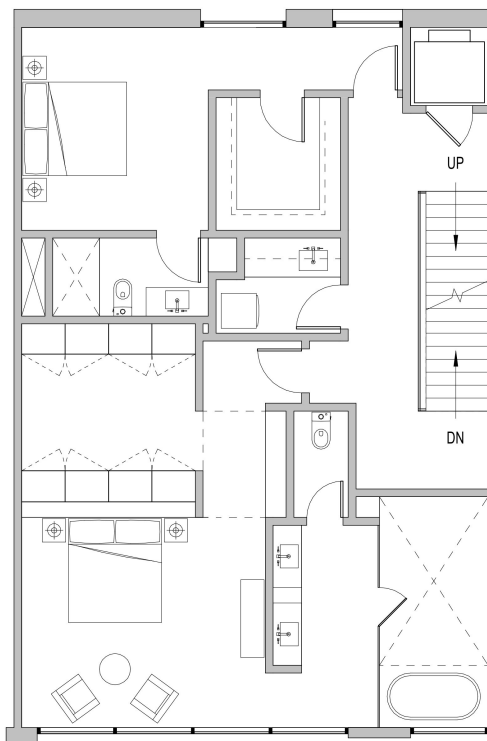
LEVEL 3
