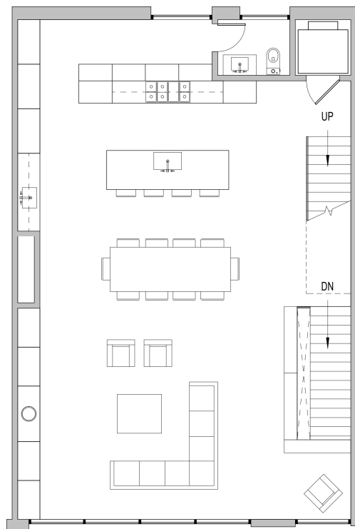
LEVEL 2
