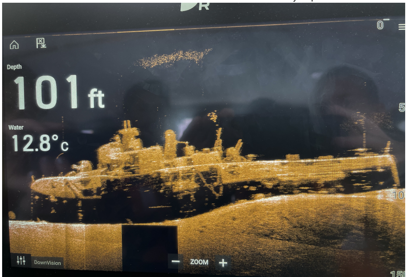
Down vision sonar of the 360' HMCS Columbia navy ship
