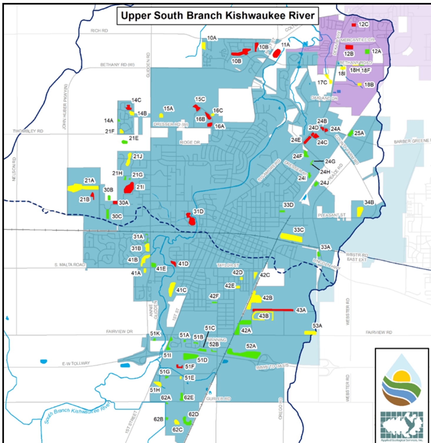
Figure 69: Detention Basin Retrofit Recommendations
