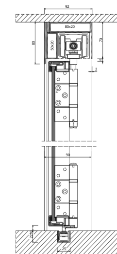
Self-contained bottom guide (located in the floor)
