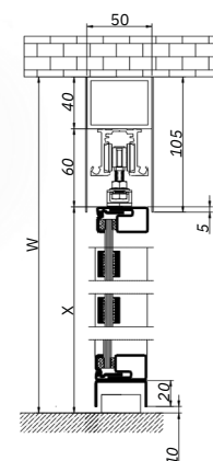
Installation to the ceiling (Standard System)
