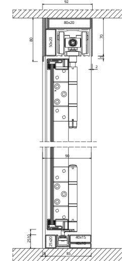
Vertical section (bottom rail on the floor)
