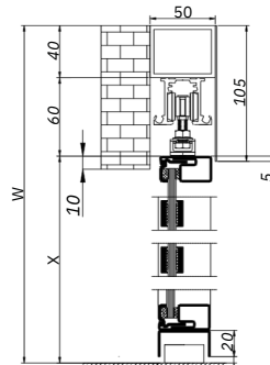
Installation to the wall/lintel (Standard System)
