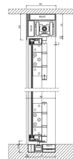
Vertical section (bottom rail recessed into the floor)
