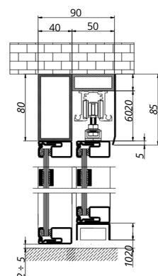
Installation to the ceiling (Standard System - sash+fix)
