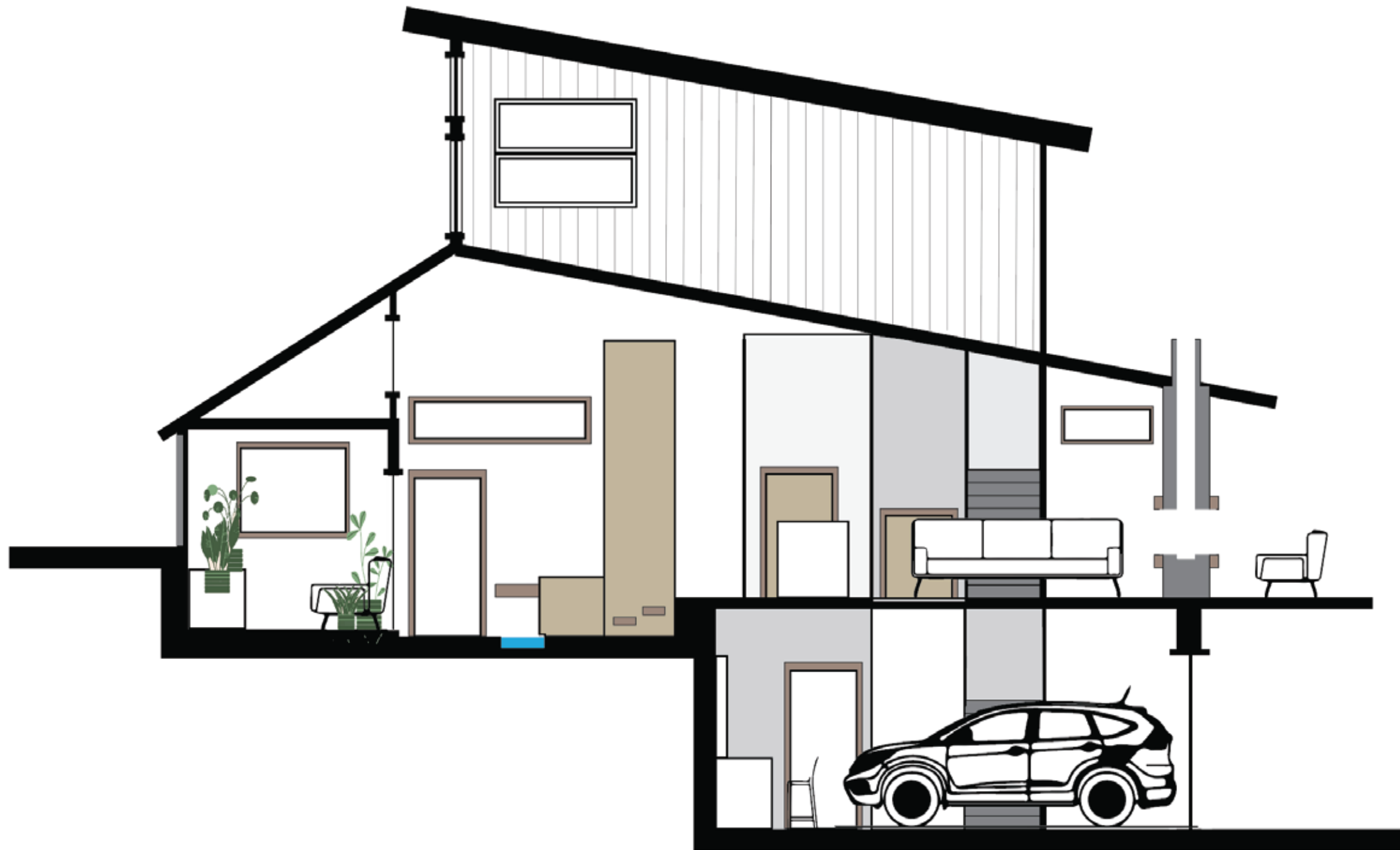
East Elevation Section Cut
