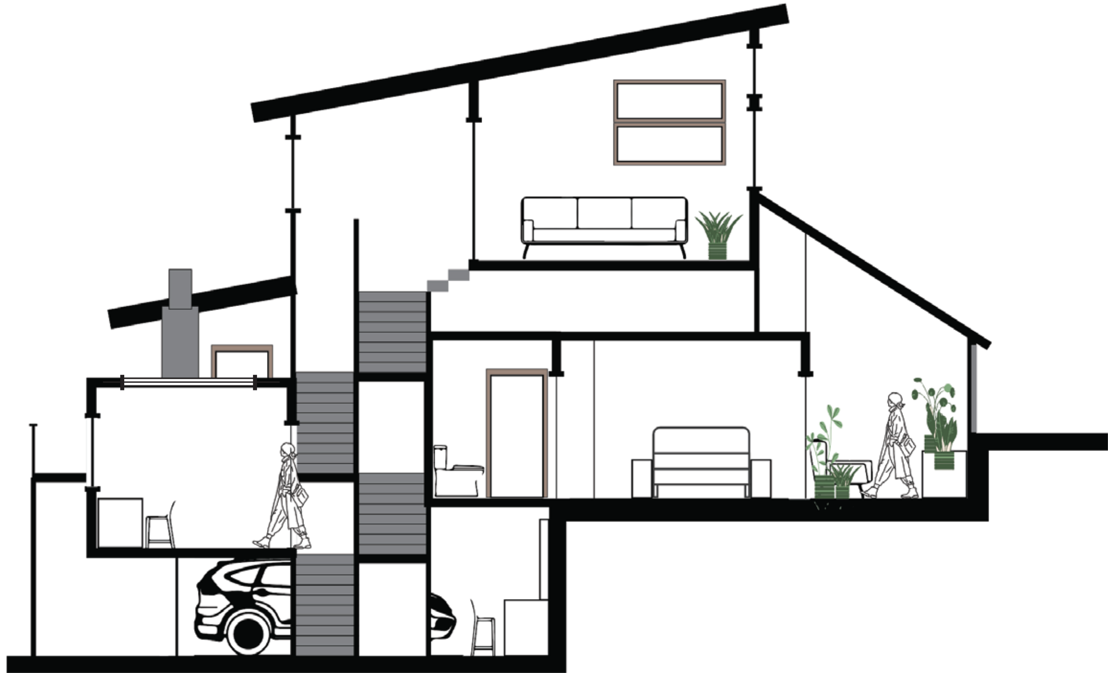
West Elevation Section Cut
