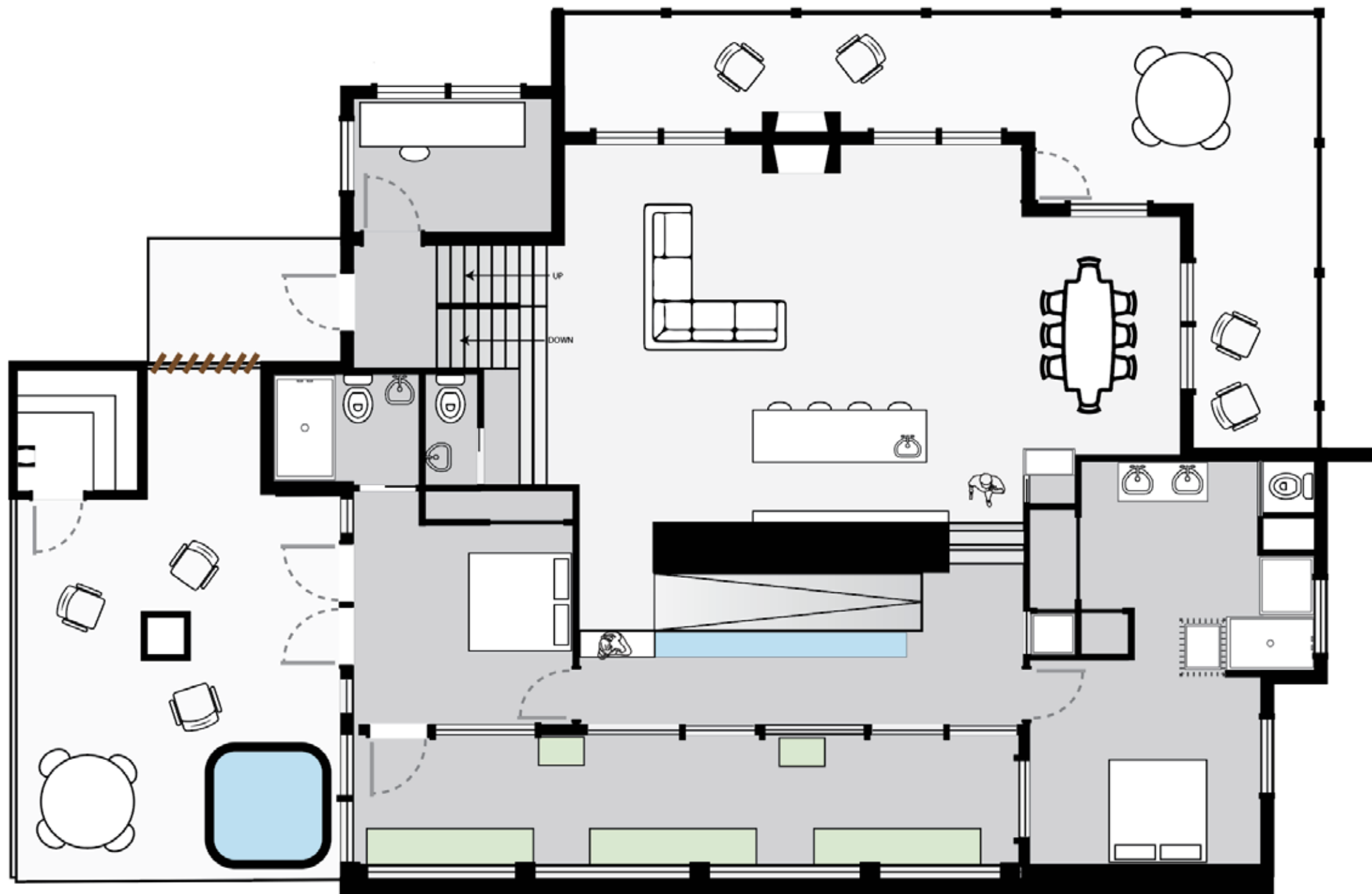
Main Levels Plan
