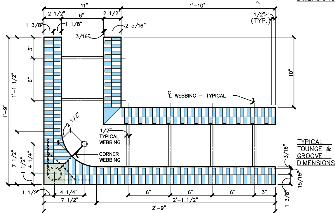
1 02 90° REVERSIBLE CORNER TOP / BOTTOM VIEW SCALE: 1 1/2" = 1'-0"
