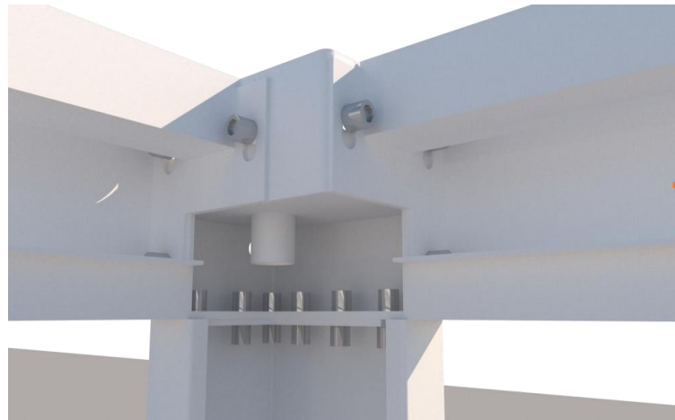
Connect top frame and column
