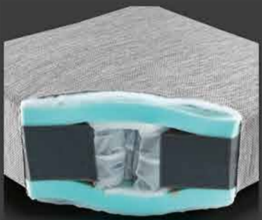
Flexible Mat Made By Combining Packed Bag Springs And Special Rubber
