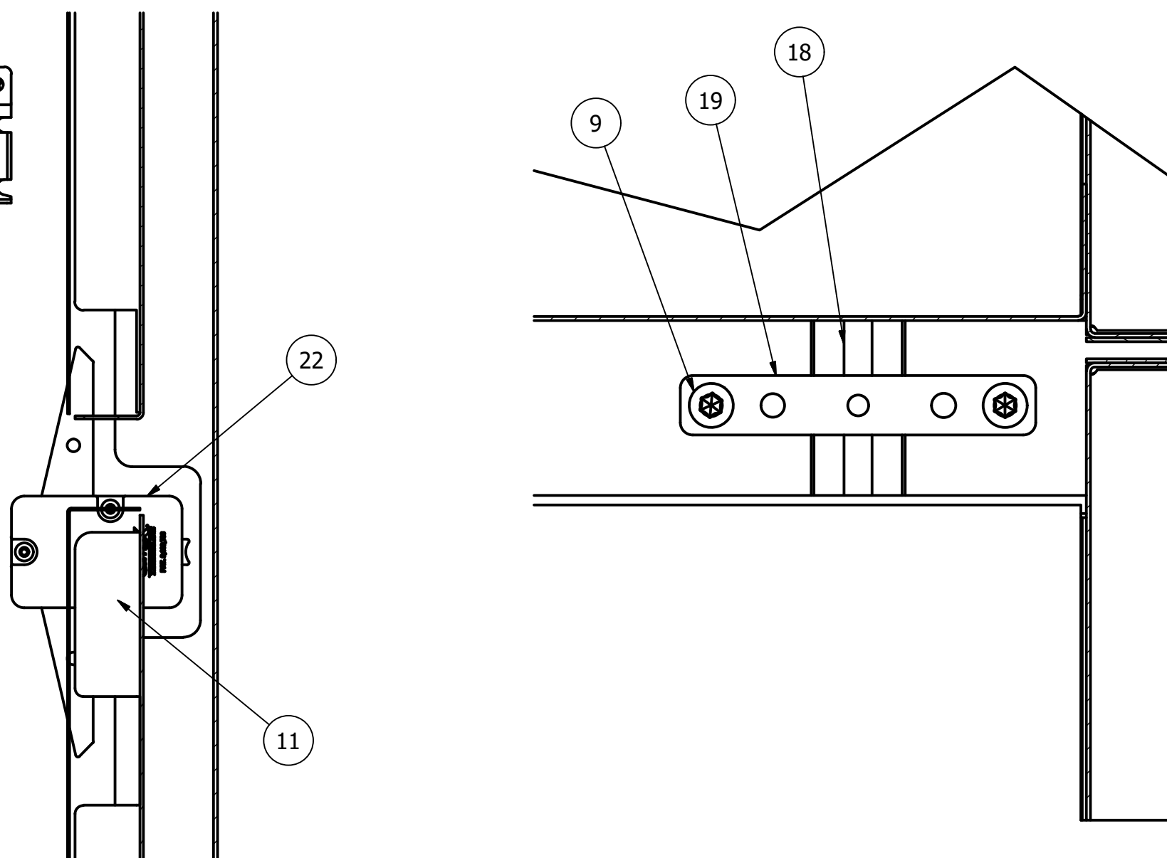
SECTION E-E SCALE 1 : 1
