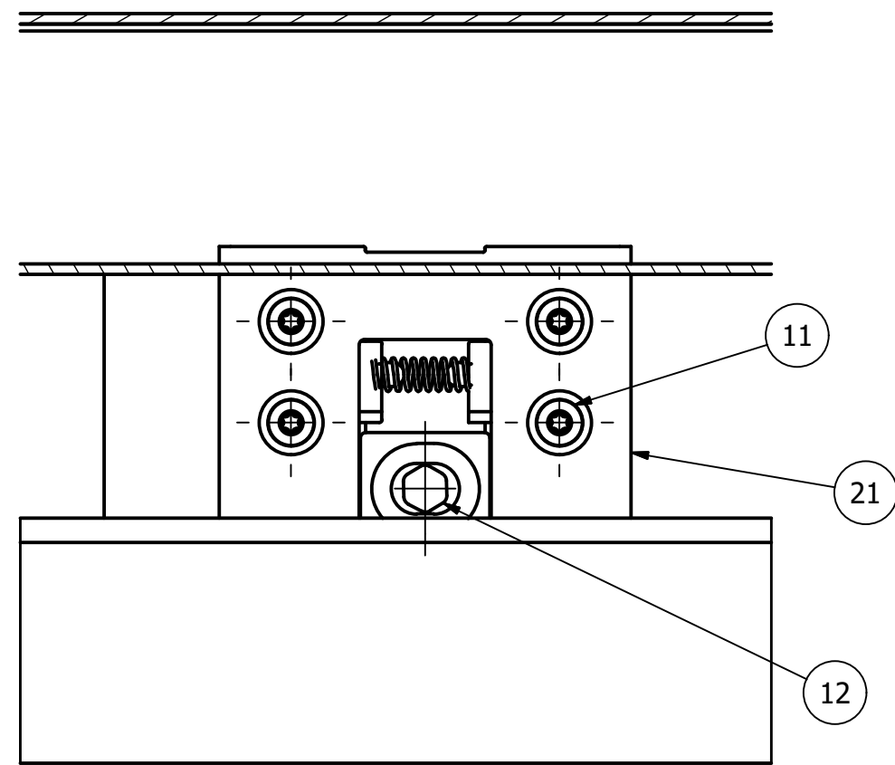
SECTION B-B SCALE 1 : 1
