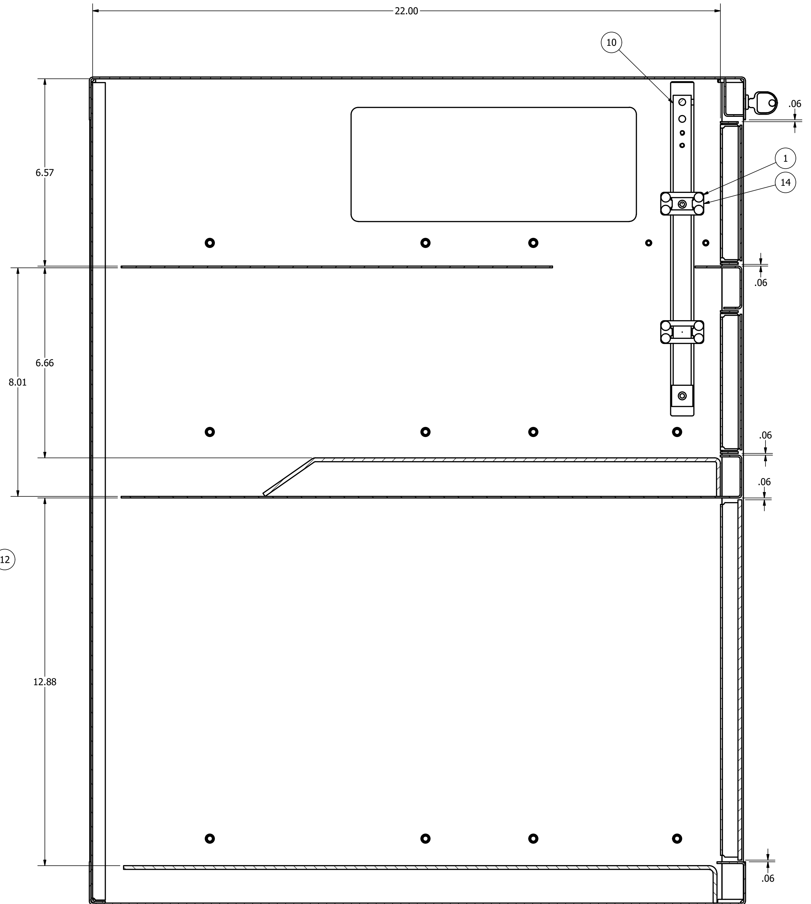
SECTION E-E SCALE 1 : 2
