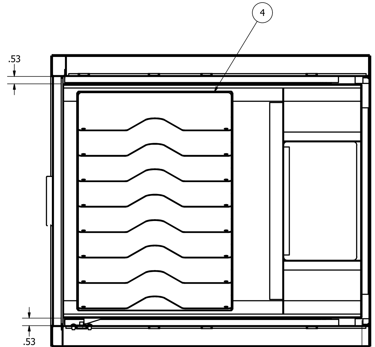
SECTION C-C SCALE 1 : 4
