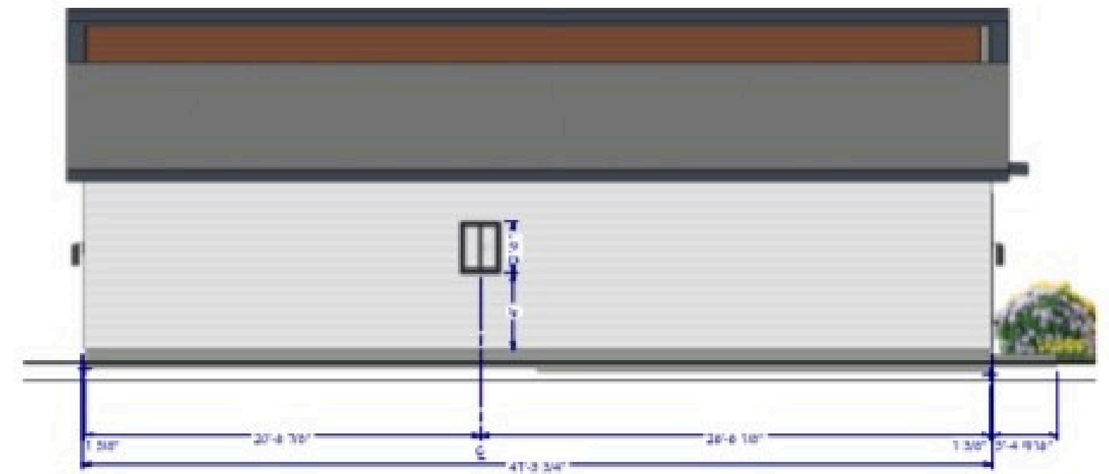
Exterior Elevation Left
