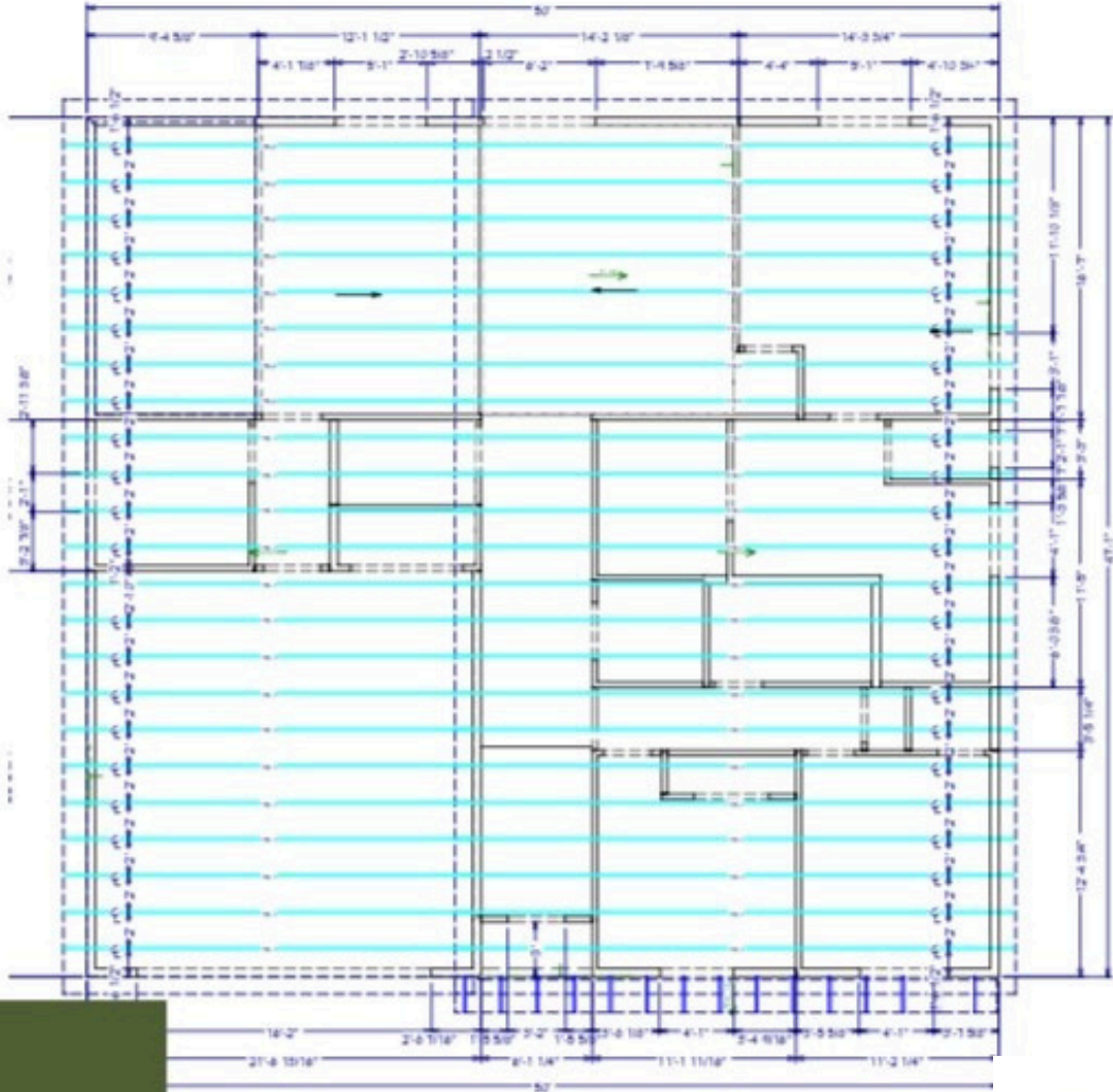
Framing, Roof Plan View
