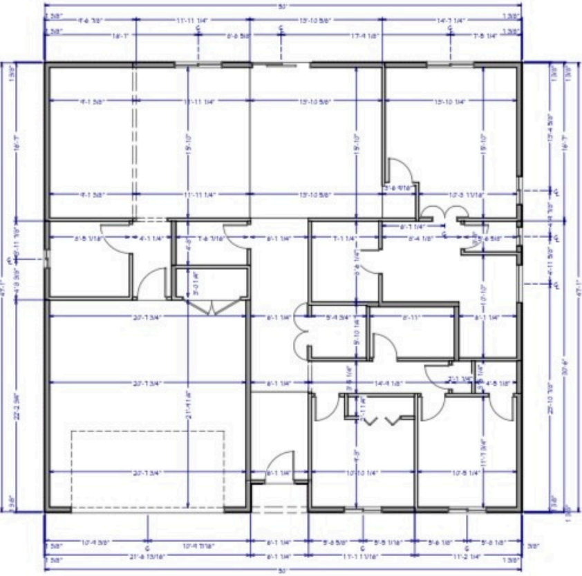
Floor Plan View Dimensioned
