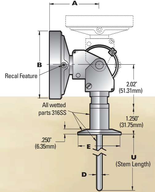
ADJUSTABLE MOUNT (shown with Tri-Clamp®)
