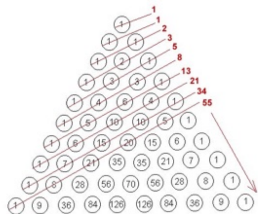
Figure 12 Pascal's Triangle
