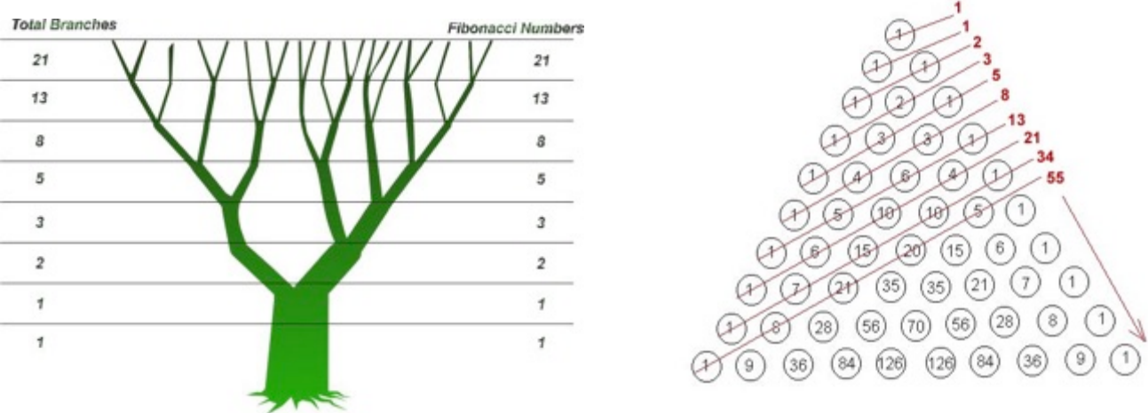
Figure 12 Pascal's Triangle
