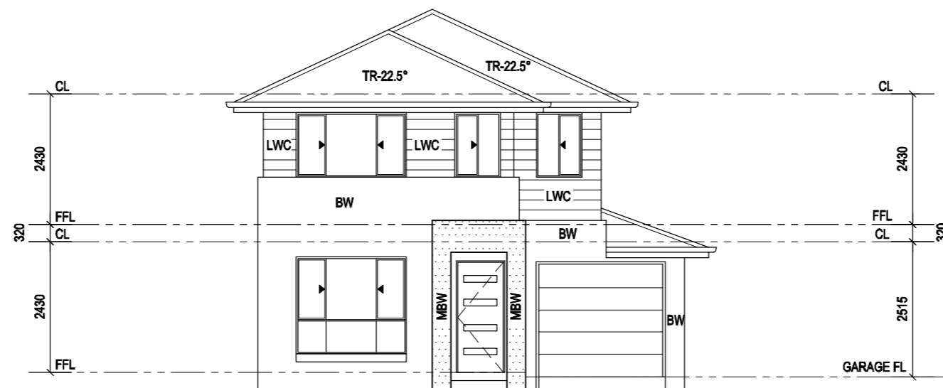
FRONT FACADE OPTION 1
