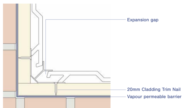
Internal Corner - Vertical Installation
