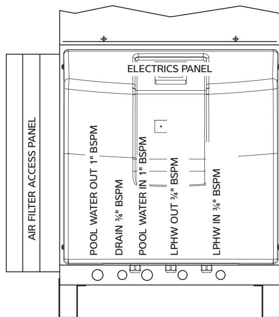
Variheat with RF pipe connections
