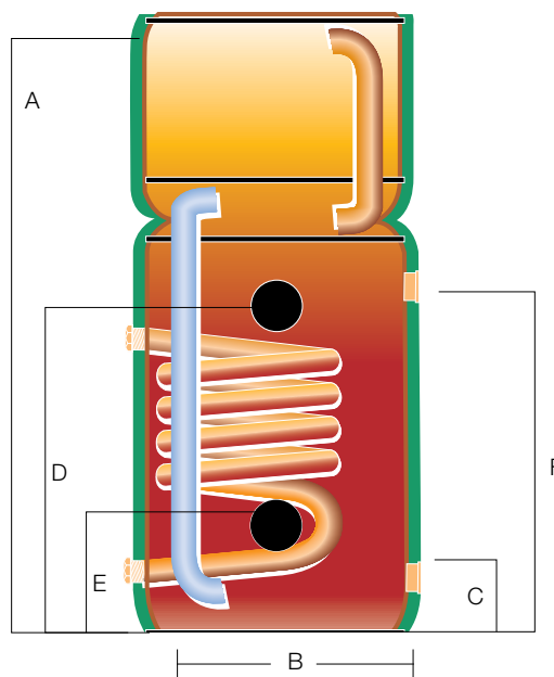
Indirect Maxistore combination unit
